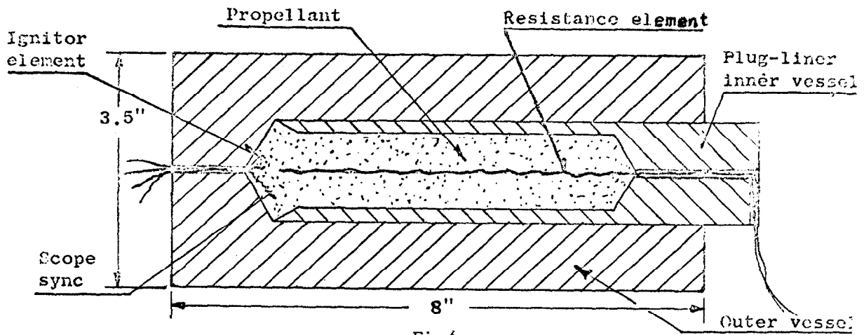
Self-sealing pressure vessel
